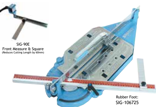
SIG-90LB Swivelling Calibrated Arm
